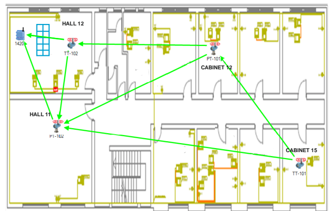
Figure 10. Mesh network
