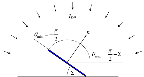
Figure 2. Cylindrical model for calculating diffuse radiation on a collector
