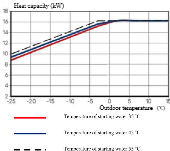
Figure 6. Capacity of the Nibe F2120-20 heat pump depending on the outdoor temperature and heating water temperature
