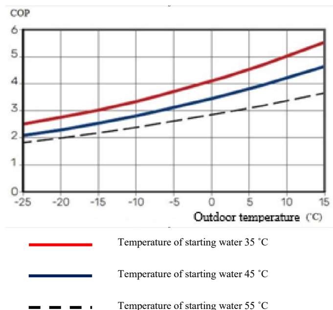
Figure 7. COP of the Nibe F2120-20 heat pump depending on the outdoor temperature and heating water temperature
