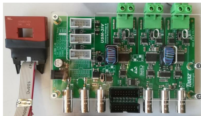
Figure 11. USM-3IV measurement electronic module.
