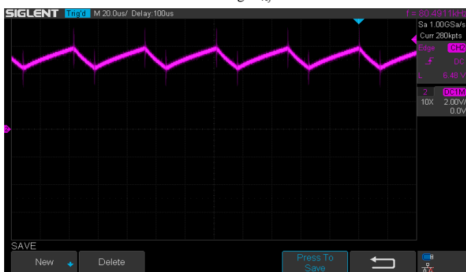
Figure 20. Inductor current of the buck converter in steady state, for the reference voltage v_{ref} = 20 V.
