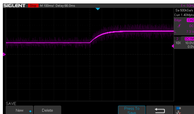
Figure 22. Output voltage of the buck converter during the step transition of the reference voltage from 10 V to 20 V.
