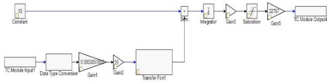
Figure 13. Control model in the TwinCAT 3 software environment.
