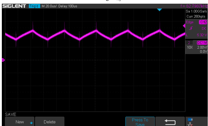
Figure 19. Inductor current of the buck converter in steady state, for the reference voltage v_{ref} = 15 V.
