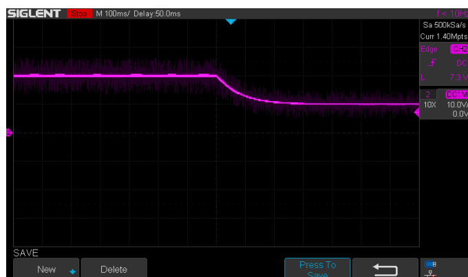
Figure 23. Output voltage of the buck converter during the step transition of the reference voltage from 20 V to 10 V.
