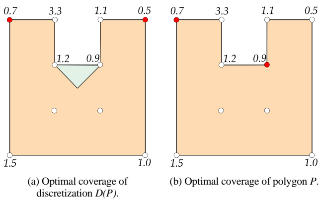
Figure 2. Optimal coverage of discretization D(P) does not imply a coverage of polygon P .
